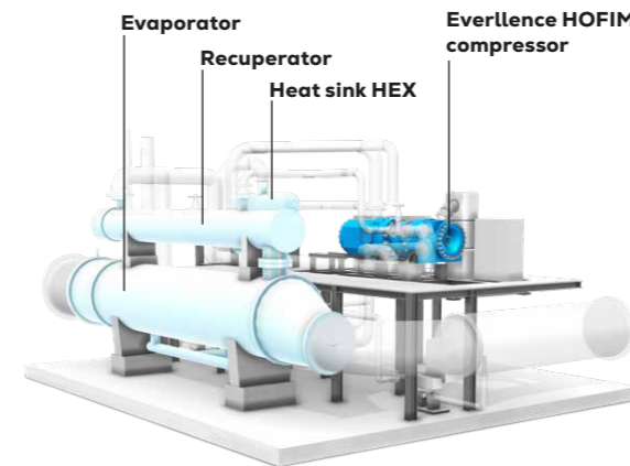
Transcritical compression cycle (TCC)
